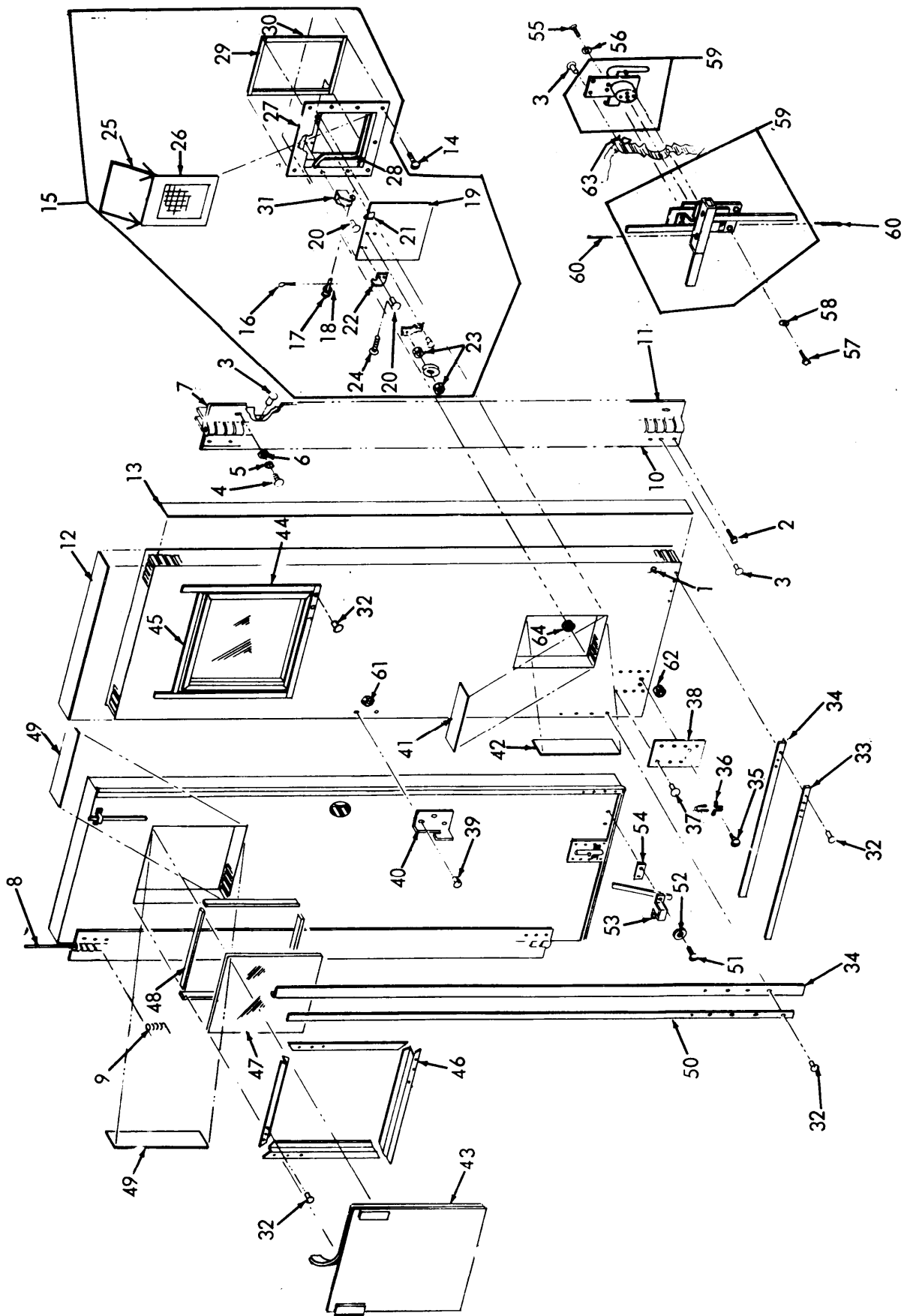
Figure 7. Door
